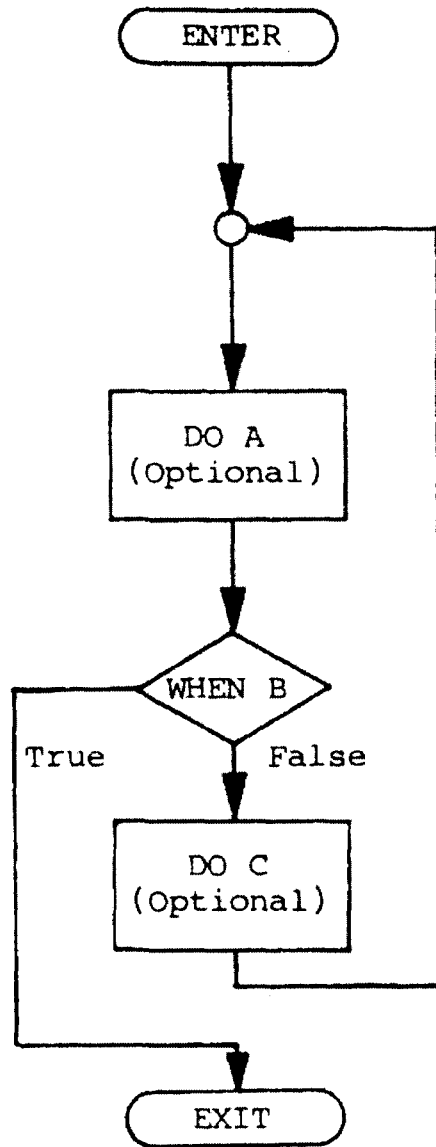
Figure 4-6, "General LOOP"
